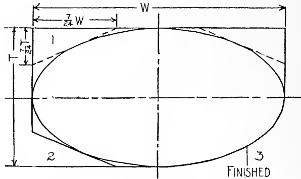
FIG. 557. LAY-OUT AND ELLIPSE.
